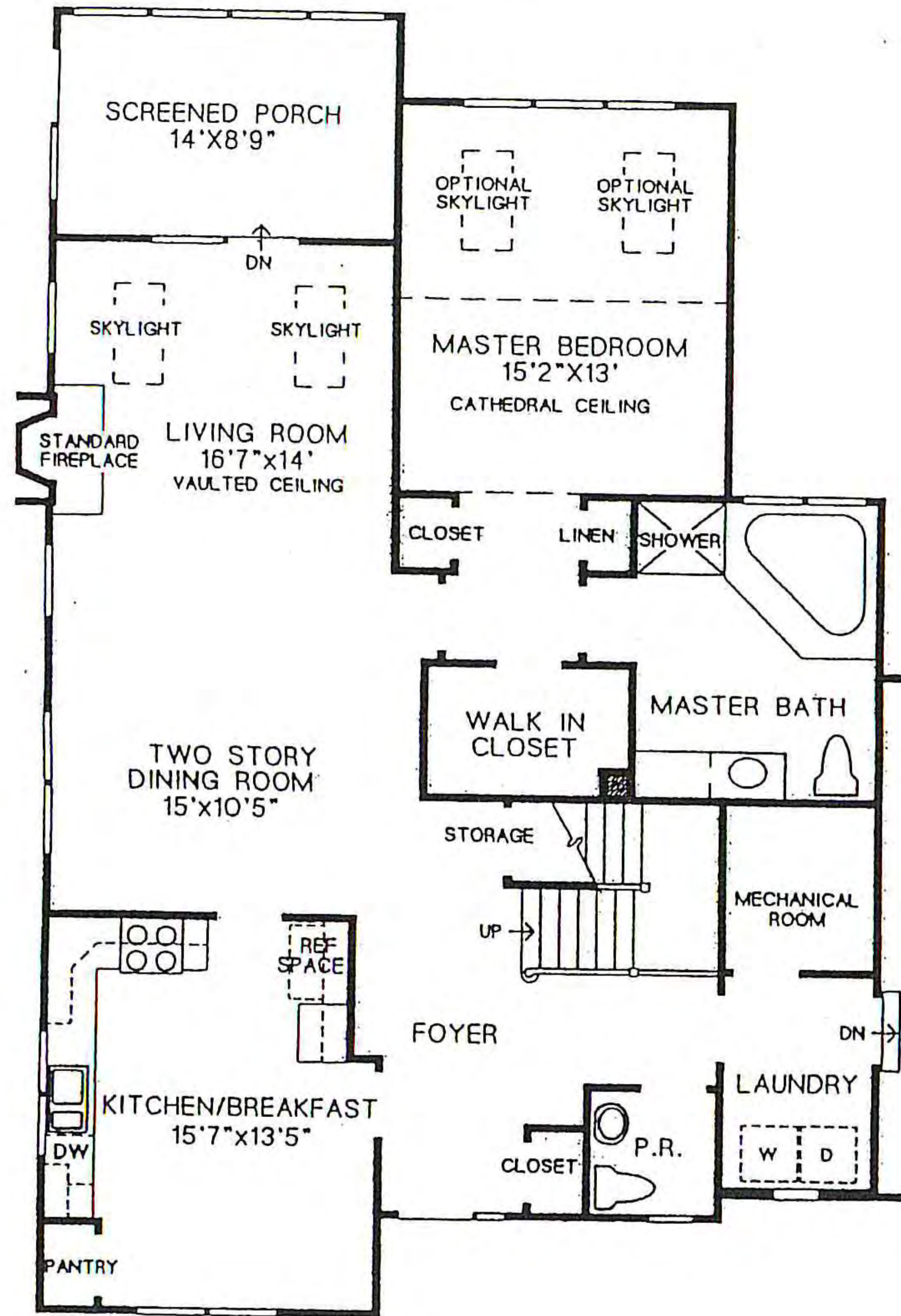
FIRST FLOOR
